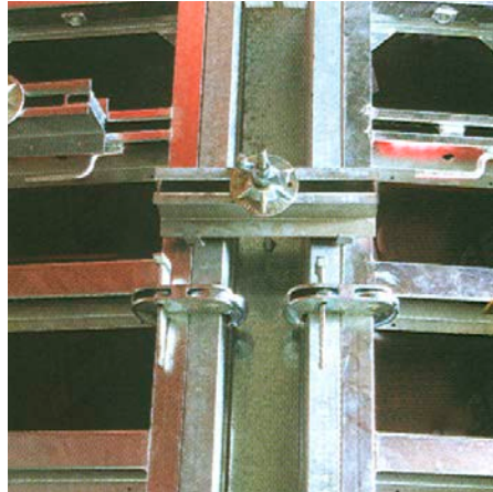
Uni Waler 40 Part No. 8359
