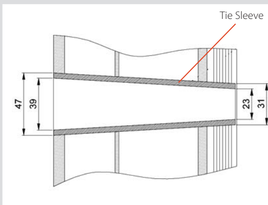
Each STERLING Panel has four tie hole sleeves within perimeter members of the galvanized frame. Tie hole sleeves are tapered for easier positioning and placing of tie rods.
