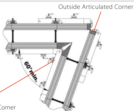
View of Inside Articulated Corner connected to Sterling Panel with Wedge Clamps.
