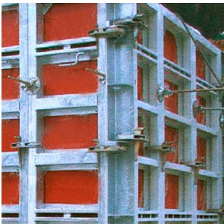
Outside Corner Part No. 8331
