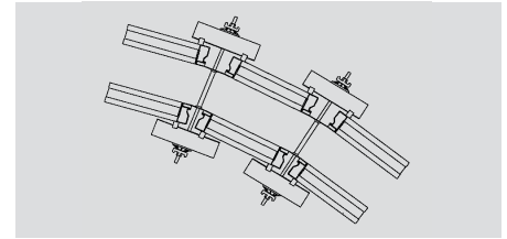
STERLING Panel 270/45 is used for forming inside and outside segmented wall forms.
