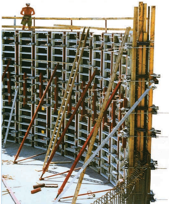
Circular Wall Form 5.7 m high ready for concrete placement.
