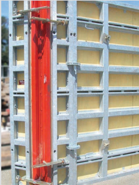
View of Outside Articulated Corner connected to two Sterling Panels with Wedge Clamps.
