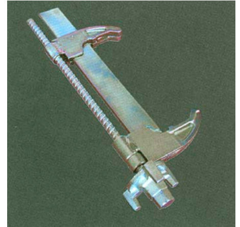
Bulkhead Coupler Clamp Part No. 8372
