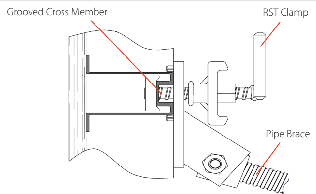
Each STERLING Panel has a Grooved Cross Member for attachment of Wall Braces, Aligner Walers or Walkway Brackets.
