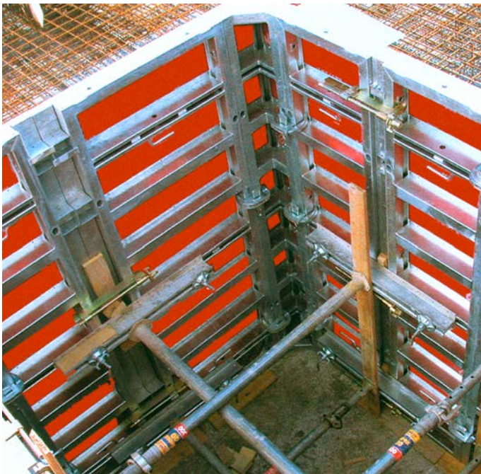
STERLING Corner Details
