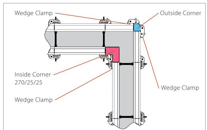
STERLING Corner Details
