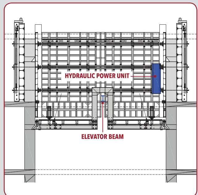
LIFT AND LOCK PLATFORM OVER ELEVATOR BEAM
